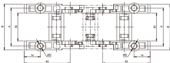
拖链安装接头 Connector of the chain
