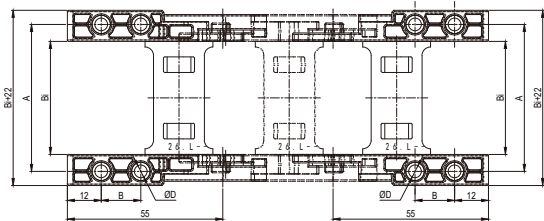
拖链示意图 Delineation of cable chain
